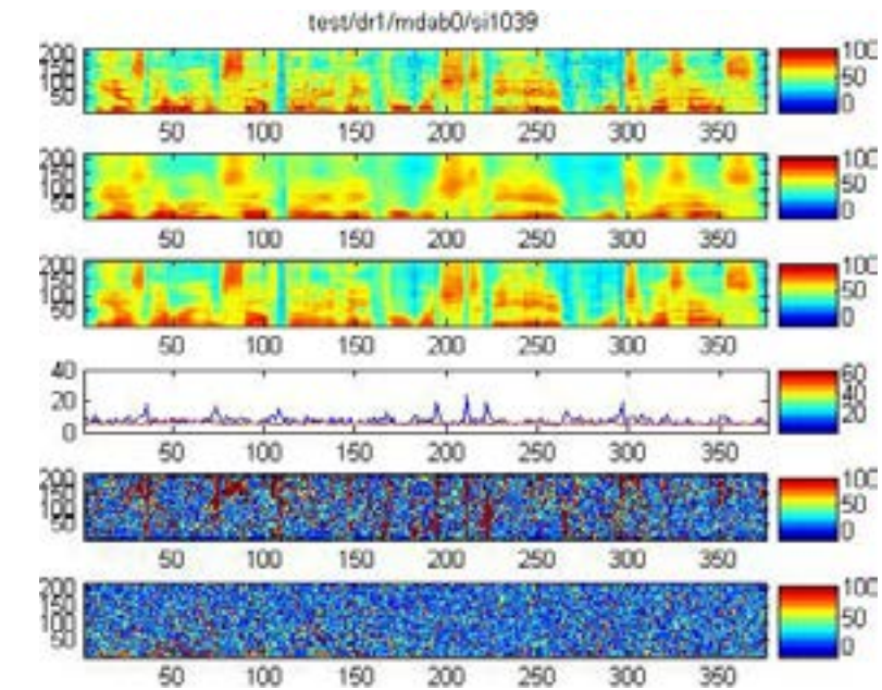
Figure 4.3: Top to bottom: The original spectrogram from the test set; reconstruction from the 312-bit VQ coder; reconstruction from the 312-bit autoencoder; coding errors as a function of time for the VQ coder (blue) and autoencoder (red); spectrogram of the VQ coder residual; spectrogram of the deep autoencoder’s residual. [after [100], @Elsevier].
