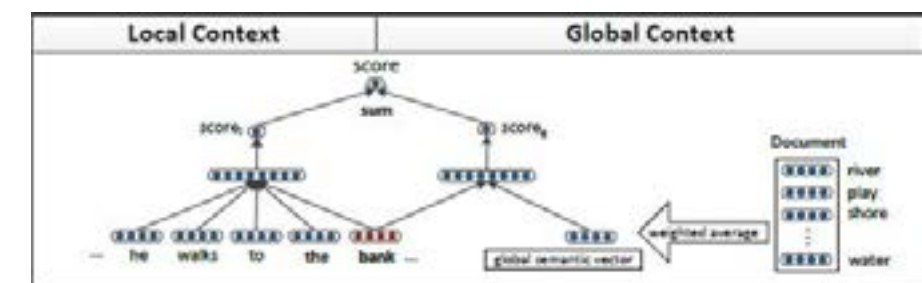
Figure 8.4: The extended word-embedding model using a recursive neural network that takes into account not only local context but also global context. The global context is extracted from the document and put in the form of a global semantic vector, as part of the input into the original word-embedding model with local context. Taken from Figure 1 of [169]. [after [169], @ACL].
