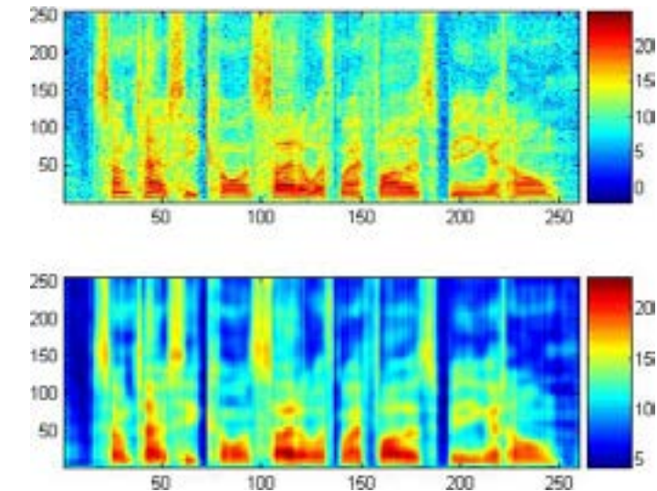
Figure 4.5: Same as Figure 4.4 but with a different TIMIT speech utterance.
