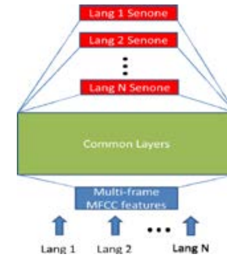
Figure 11.5: A DNN architecture for multilingual speech recognition. [after [170], ©IEEE].
