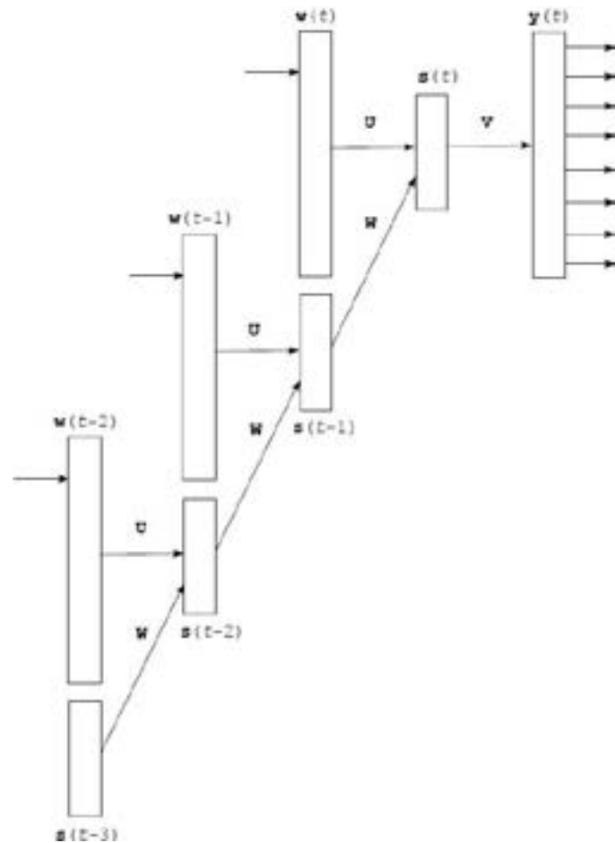
Figure 8.2: During the training of RNNLMs, the RNN unfolds into a deep feed-forward network; based on Figure 3.2 of [245].
