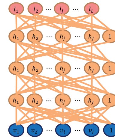
Figure 5.2: An illustration of the DBN-DNN architecture.
