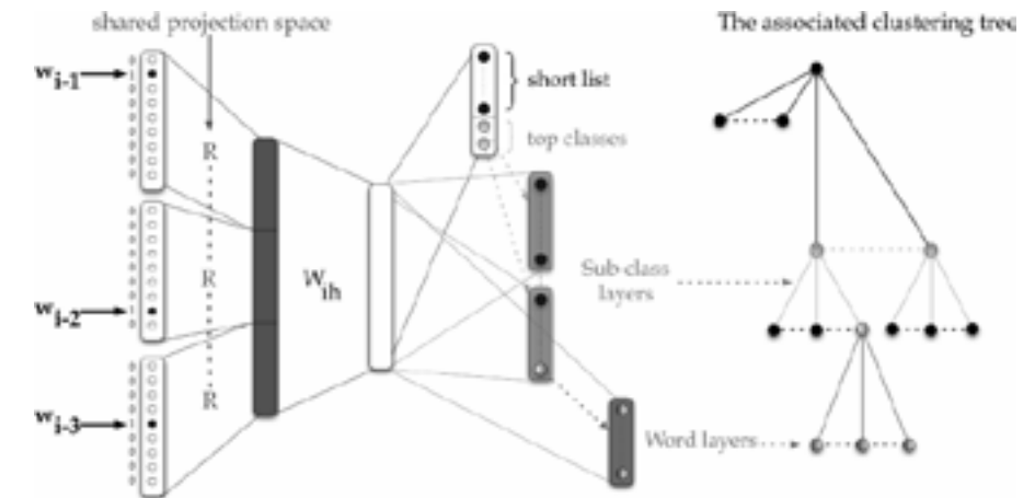
Figure 8.1: The SOUL-NNLM architecture with hierarchical structure in the output layers of the neural network [after [207], ©IEEE].
