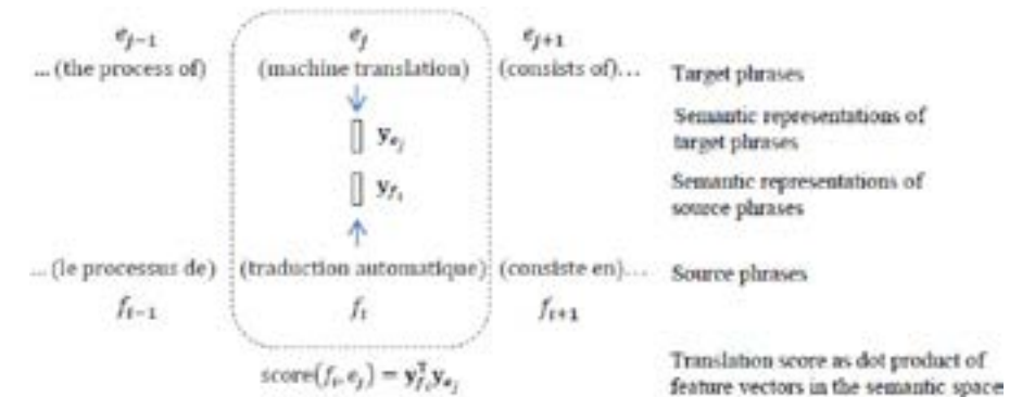
Figure 8.5: Illustration of the basic approach reported in [122] for machine translation. Parallel pairs of source (denoted by f ) and target (denoted by e ) phrases are projected into continuous-valued vector representations (denoted by the two y vectors), and their translation score is computed by the distance between the pair in this continuous space. The projection is performed by deep neural networks (denoted by the two arrows) whose weights are learned on parallel training data. [after [121], @NIPS].
