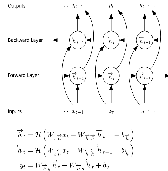
Figure 7.3: Information flow in the bi-directional RNN, with both diagrammatic and mathematical descriptions. W 's are weight matrices, not shown but can be easily inferred in the diagram. [after [136], ©IEEE].
