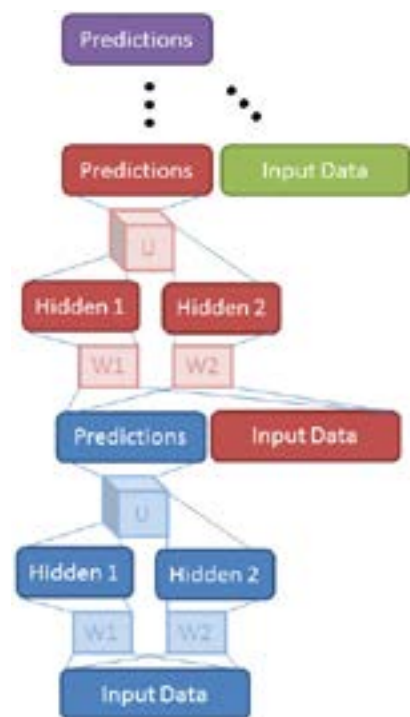
Figure 6.3: Stacking of TDSN modules by concatenating prediction vector with input vector. [after [180], ©IEEE].
